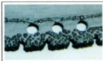
Shown: Laser-welded segments with large sized industrial type grit.
